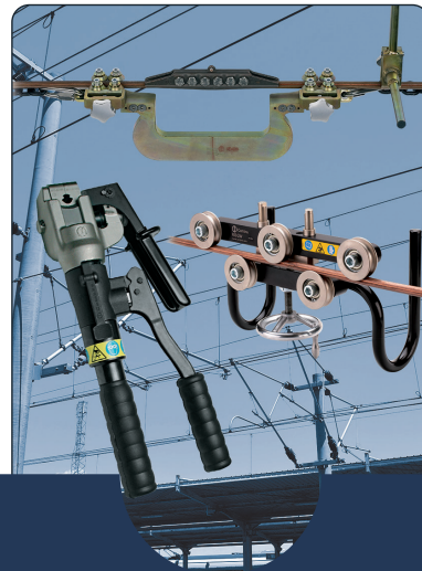
Catenary tools
